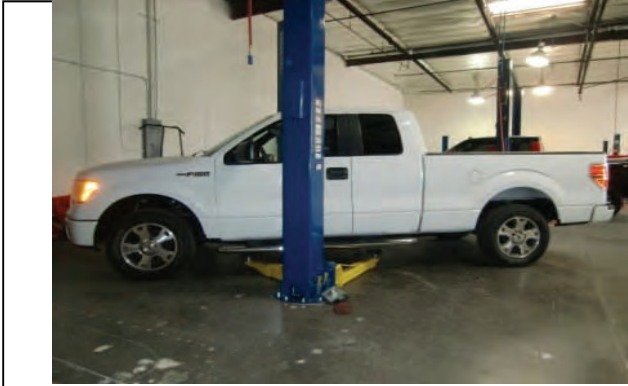
Measure vehicle on level surface and raise by frame
